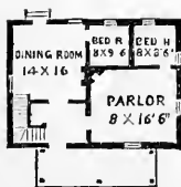
FIG. 32.—FIRST FLOOR.
