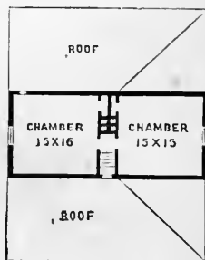
FIG. 100.—SECOND FLOOR.
