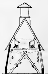
FIG. 135. SECTION.
