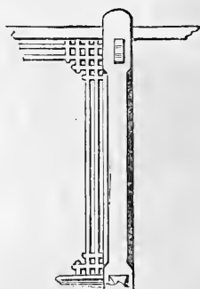
FIG. 175.—DETAIL OF ARBOR.
