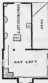
FIG. 160.—SECOND FLOOR.
