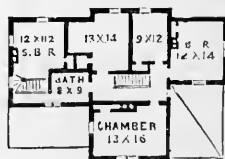
FIG. 131.—SECOND FLOOR.
