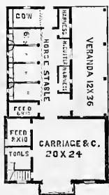
FIG. 159.—FIRST FLOOR.
