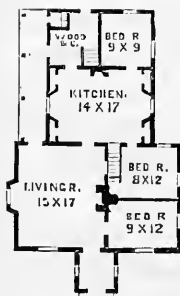
FIG. 155.—FIRST FLOOR.
