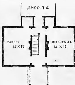
FIG. 17.—FIRST FLOOR.
