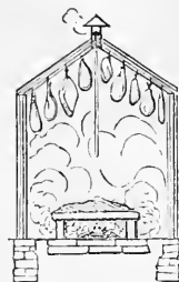
FIG. 113.—SECTION.
